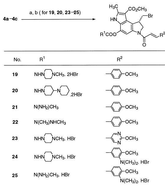
Scheme 3. (a) (1) HBr, CH 3 CN, (2) 4-nitrophenyl chloroformate, Et 3 N, CH 2 Cl 2 , (3) The free base of R 1 H; (b) HBr.
