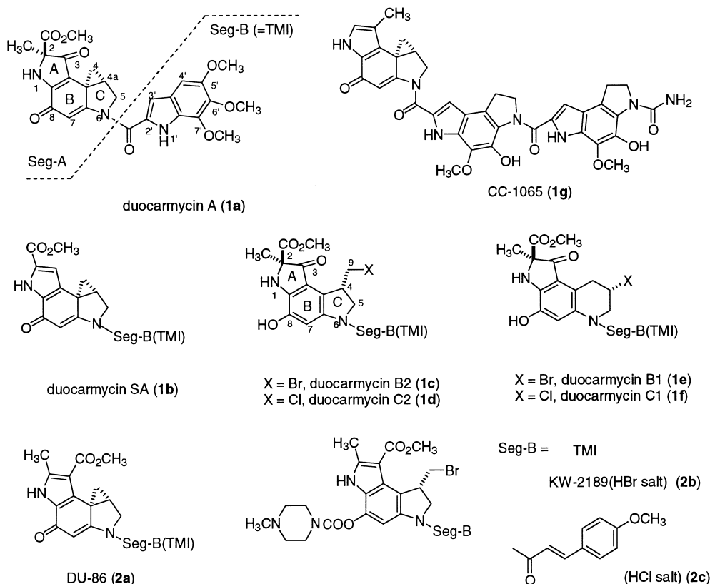
Figure 1. Structure of duocarmycins, CC-1065, and duocarmycins derivatives.
